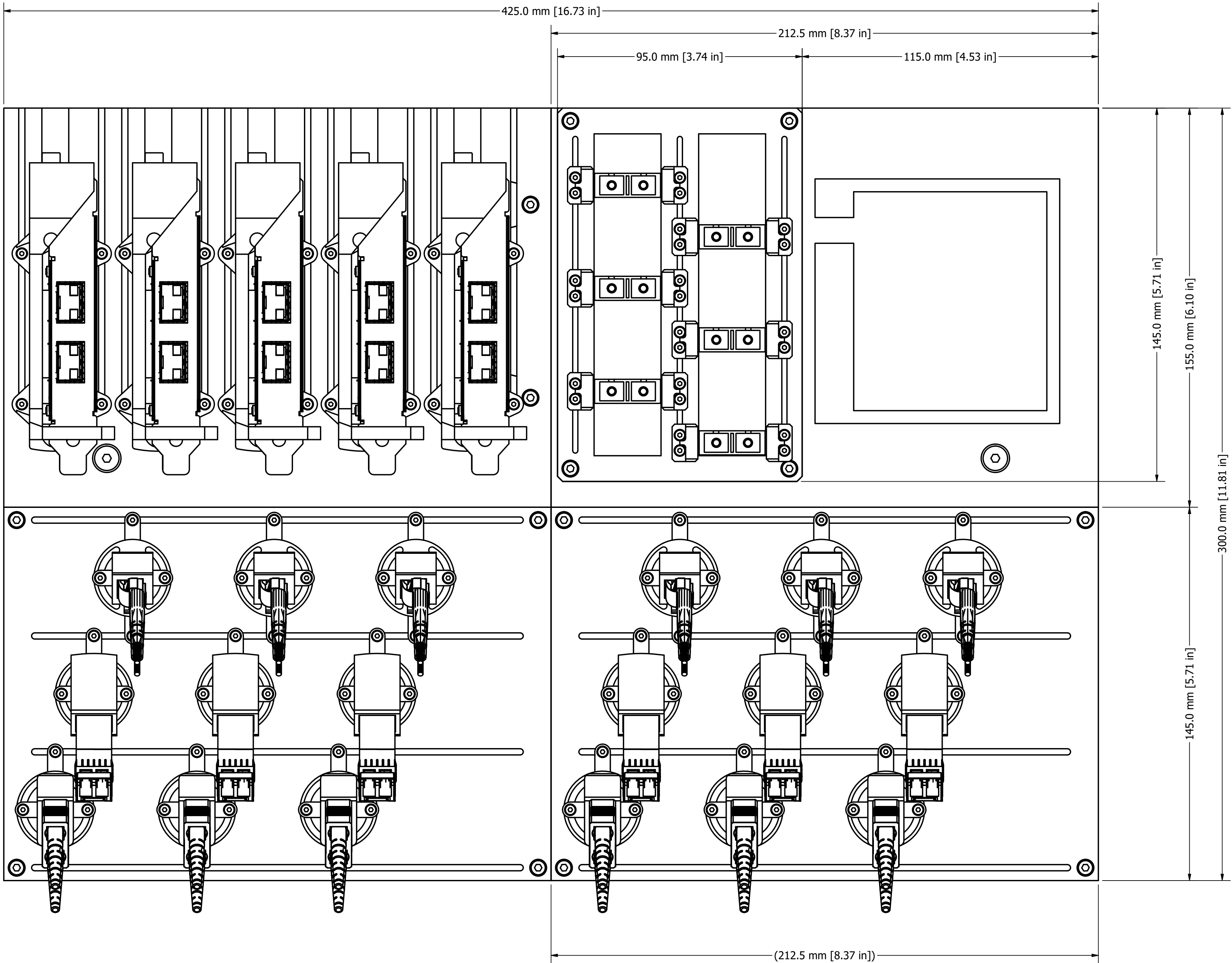
PLAN SCALE 1 / 1
